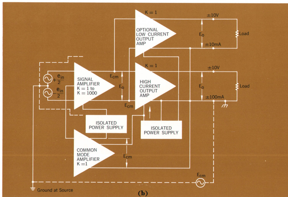
Fig. 3. The HP Model 8875A Data Amplifier (a) uses a common mode amplifier (b) to provide good common mode rejection without the use of a specially shielded power transformer.
