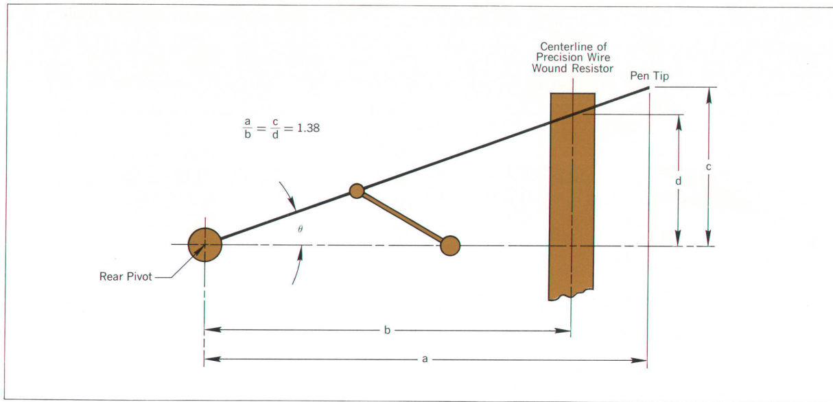
Fig. 7. Transducer near pen tip is linear. Ratio of tip motion to pickoff-wire displacement is 1.38 to 1.
