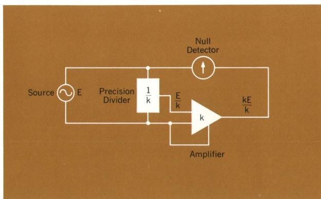
Fig. 4. Use of the bridge method of checking gain linearity of an amplifier with gain K is relatively inexpensive and rapid. Precision depends mainly upon the accuracy of the voltage divider and the sensitivity of the null detector.
